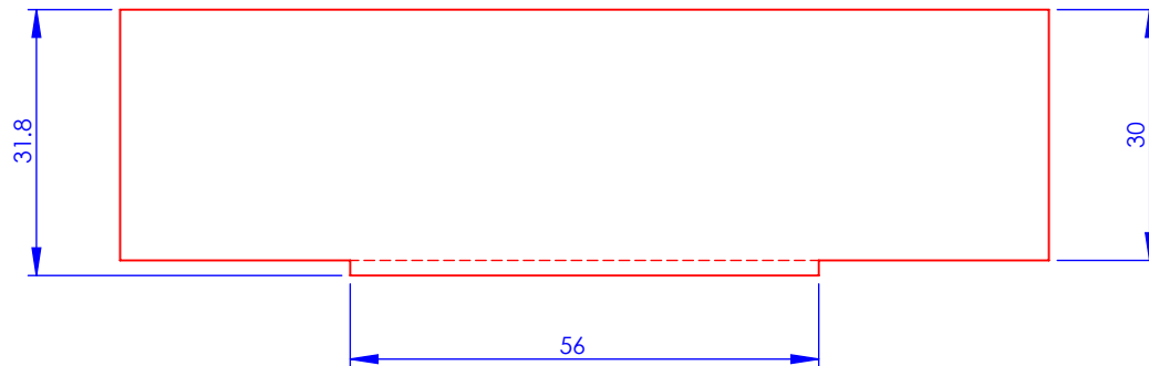
Milling top view
