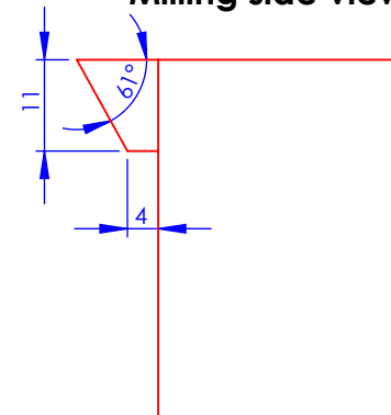
Milling side view
