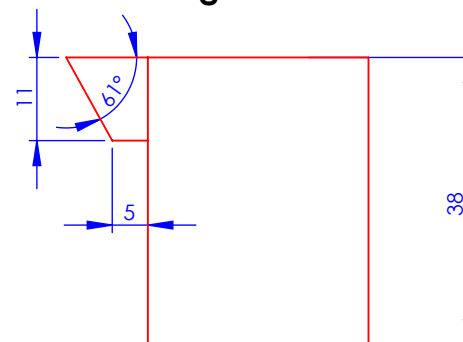
Milling side view
