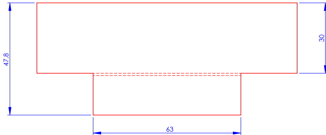
Milling front view
