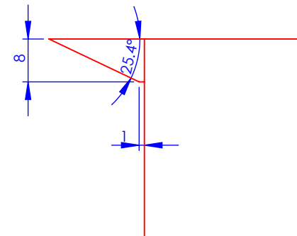
Milling side view
