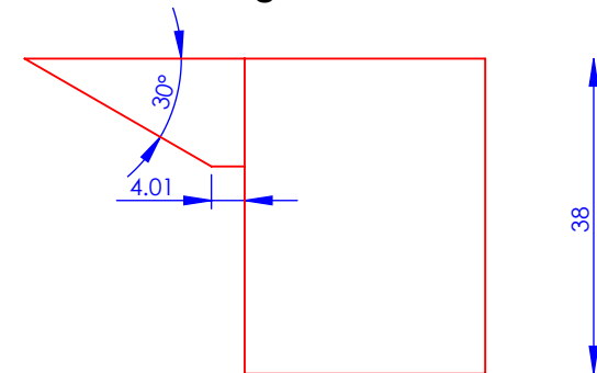
Milling side view
