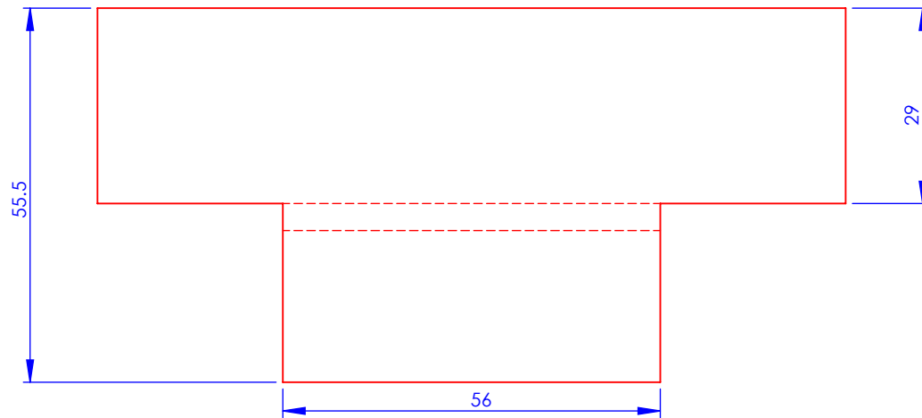
Milling top view
