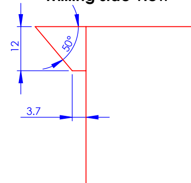
Milling side view
