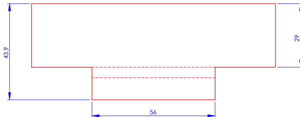
Milling front view
