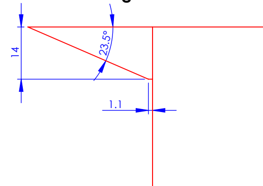
Milling side view
