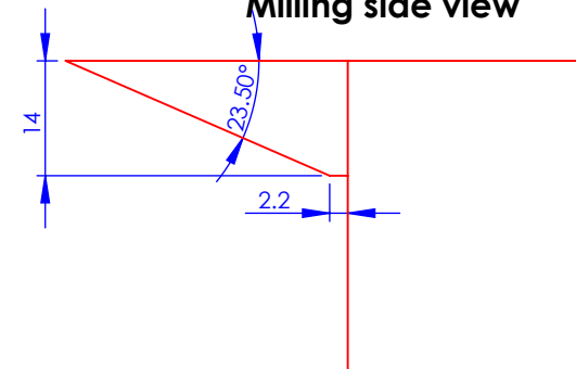
Milling side view
