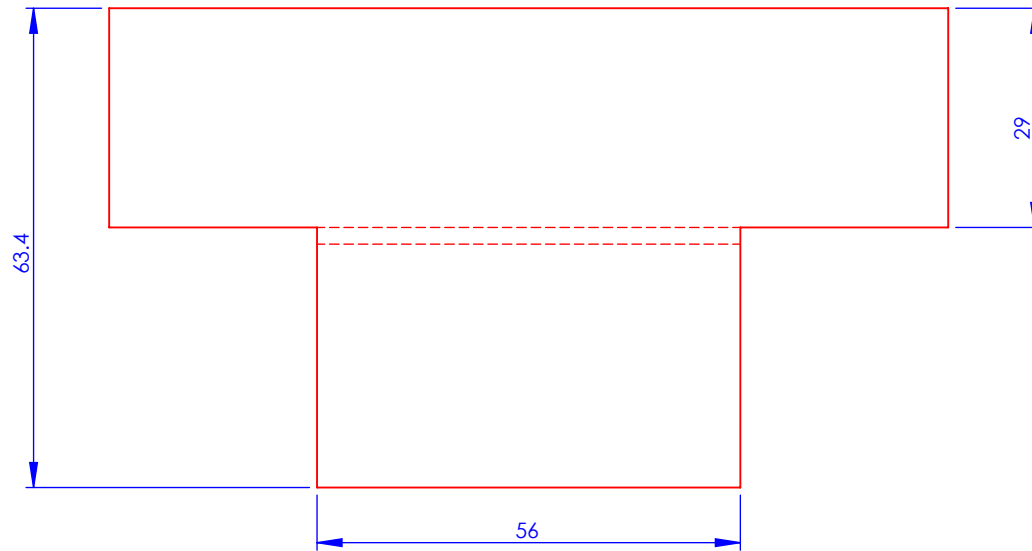
Milling front view
