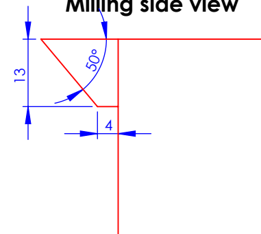
Milling side view
