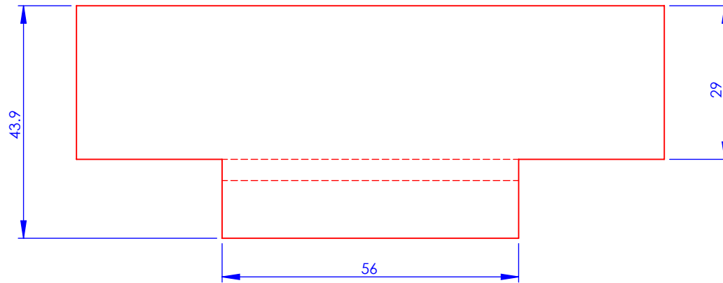
Milling top view
