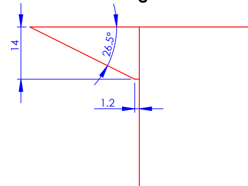
Milling side view
