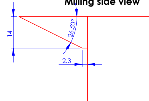
Milling side view
