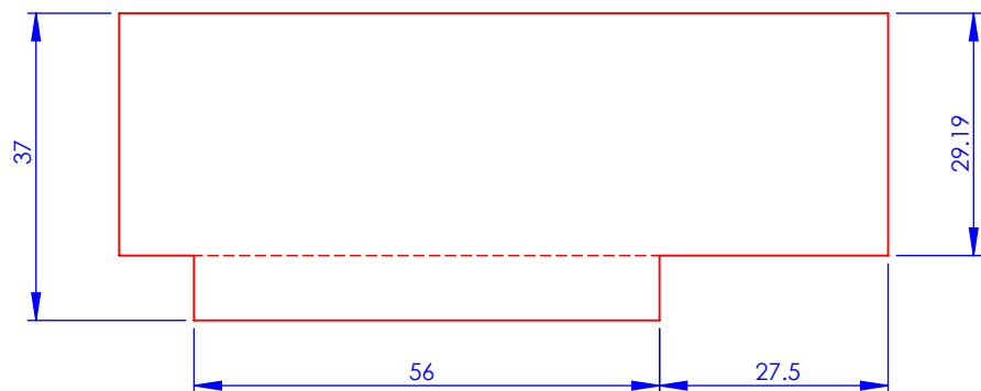
Milling top view
