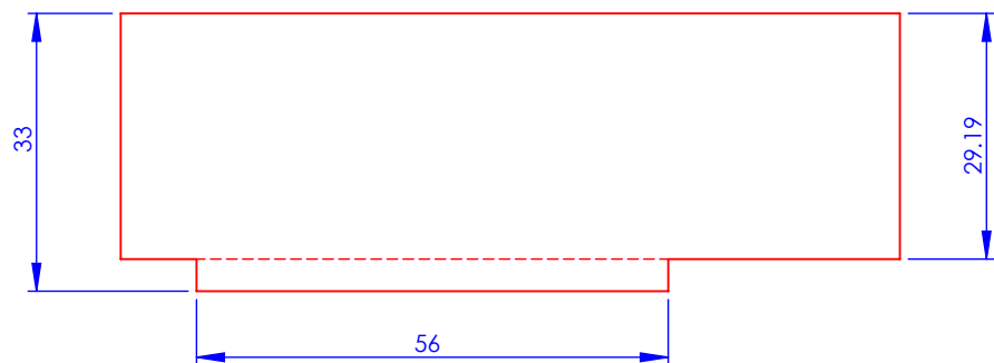
Milling top view
