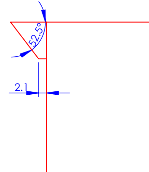
Milling side view
