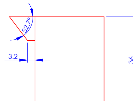
Milling side view
