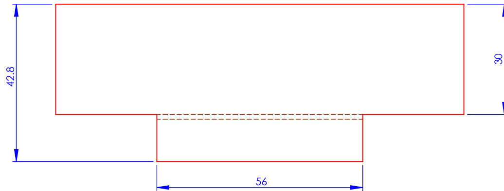
Milling front view
