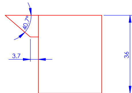
Milling side view
