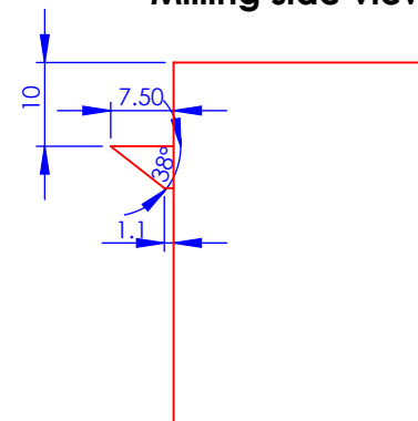
Milling side view
